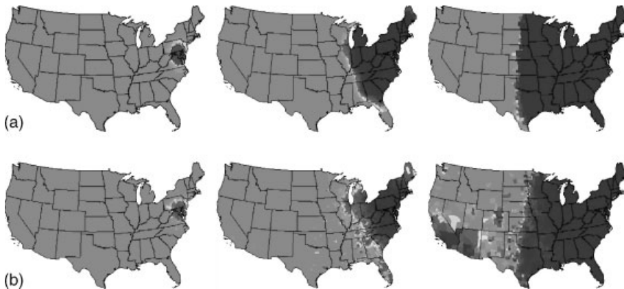
Figure 1.9 Simulation of the fractional, spatially extended SIS model (b) in the United States compared to a system with ordinary diffusion (a). Each column represents a snapshot of the time evolution of both systems. The initial outbreak in the simulations was in
