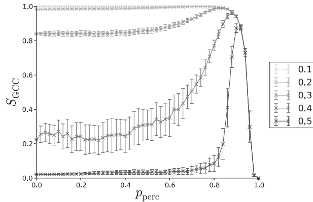
FIG. 6. The skeleton GCC, S_{\text{GCC}} , of the Random network with different salience cutoffs. For salience cutoff values > 0.3 , the S_{\text{GCC}} increases at p_{\text{perc}} \approx 0.8 and then begins decreasing at p_{\text{perc}} \approx 0.95 . The unique shape of the salience distribution of the Random network leads to different cutoffs being required for robustness.
